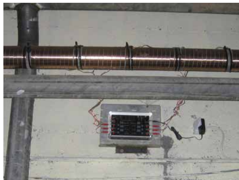
The installation of Vulcan S100 in a water meter and electricity meter production.
