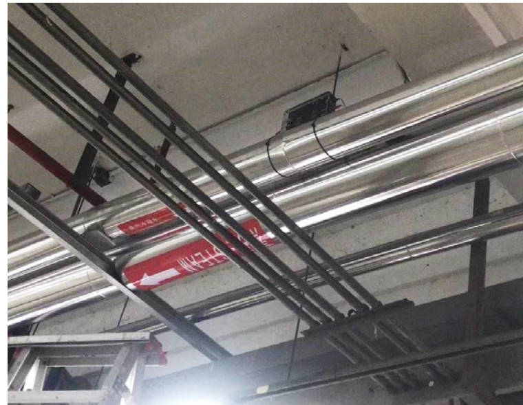
Step 2: Pipe is wrapped with insulation material, then install Vulcan S25 unit
