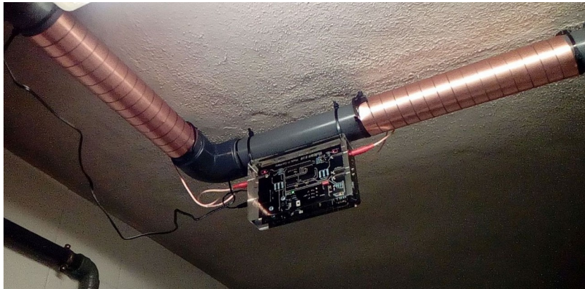
Vulcan S10 – Cold water main pipe
