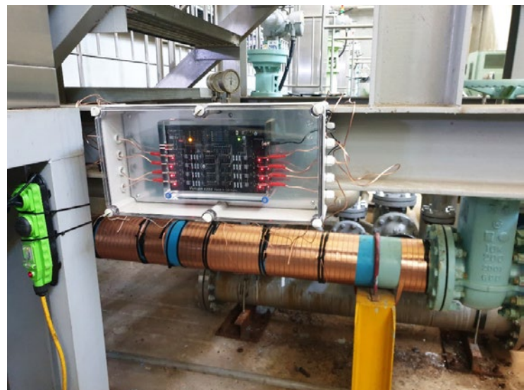
Vulcan S250 installed at K-water
